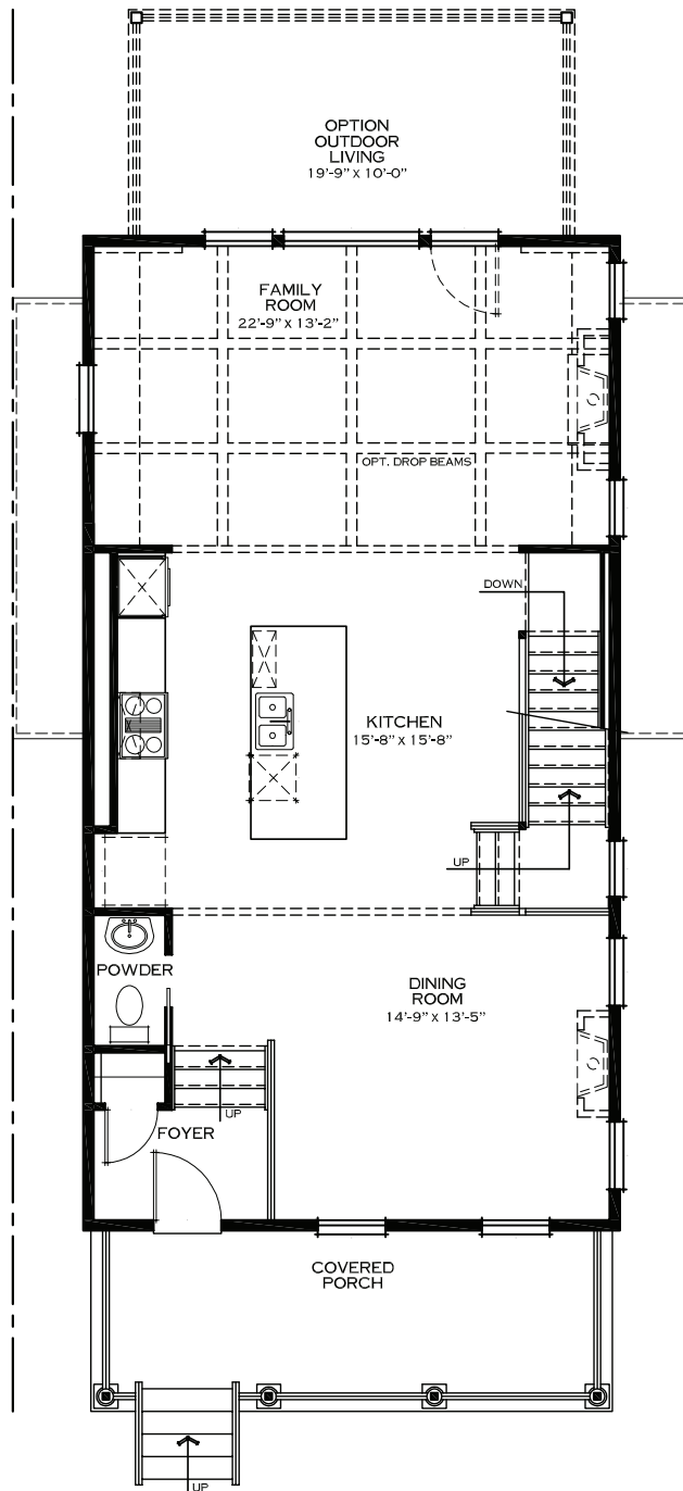
MAIN FLOOR (Second Level)
