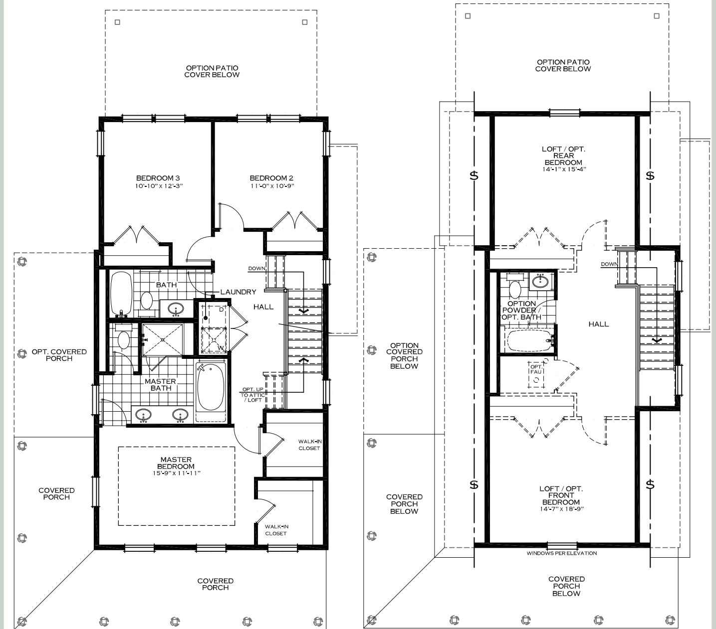
BEDROOM FLOOR (Third Level)
