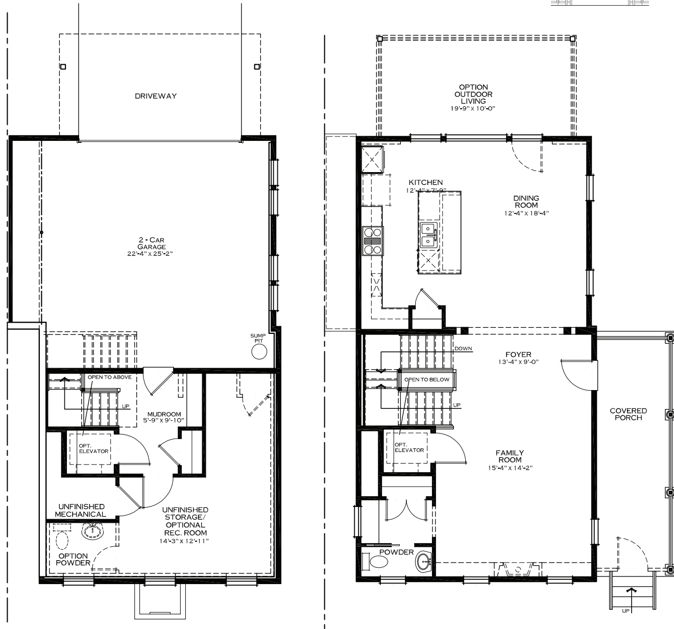
GARAGE FLOOR (First/Ground Level)
