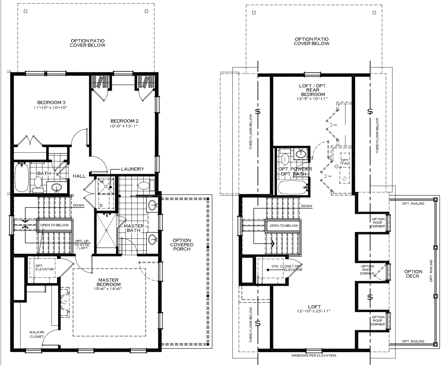
BEDROOM FLOOR (Third Level)
