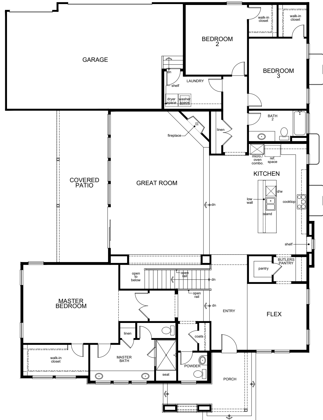
FIRST FLOOR
