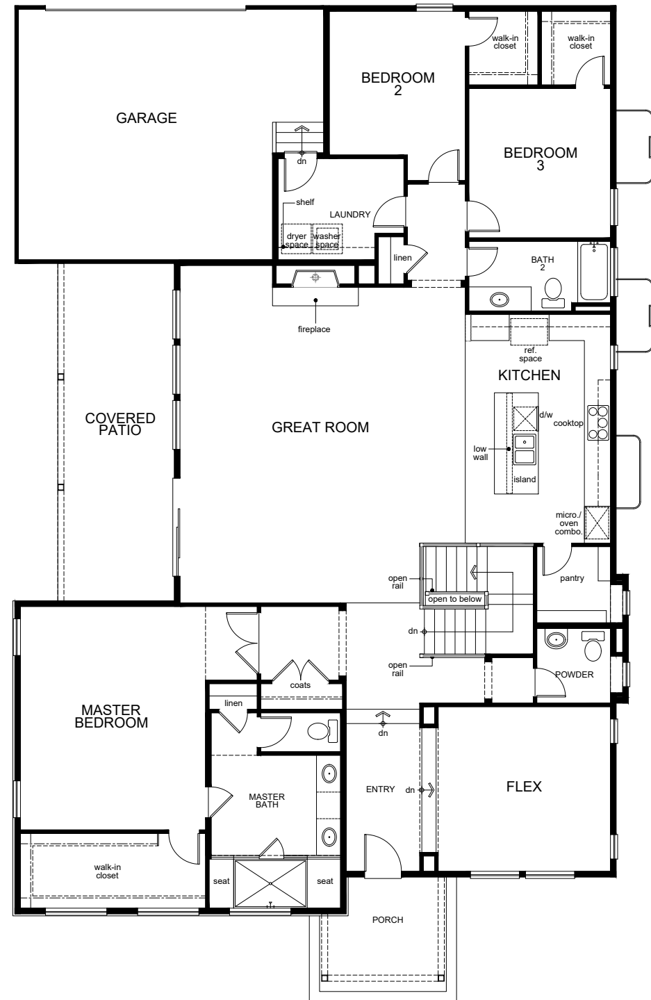
FIRST FLOOR
